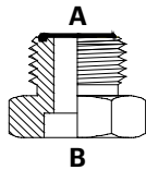
ORFSM Tube Weld
