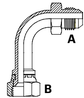
JICM x JICFS 90° Long Bend
